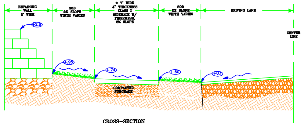
CROSS-SECTION B-B
