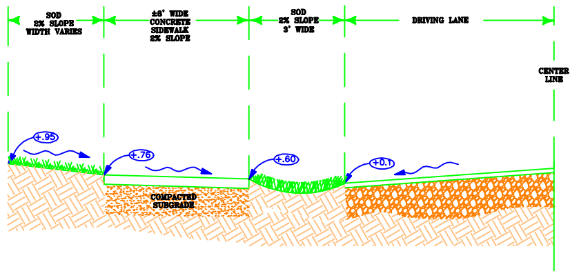
CROSS-SECTION D-D TYPICAL
