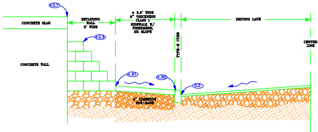
CROSS-SECTION C-C
